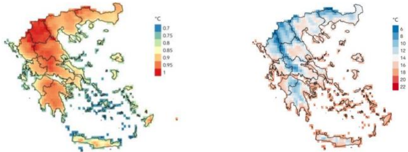
Figure 1. (a) Spatial distribution of the average annual temperature increase (°C) in the reference period 1971-2000; (b) expected differences in the spatial distribution of the average annual temperature increase (°C) during the period 2026-2045.
